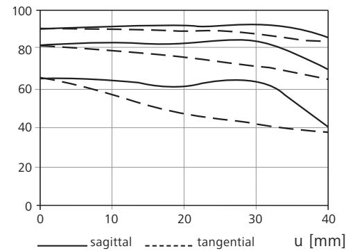
MTF [%], f-number: k = 8.0
