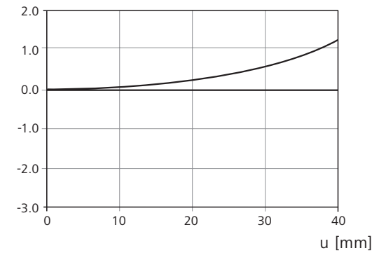
V [%], Distortion
